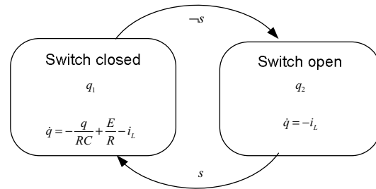
Figure 2 Open loop power conditioning system.
