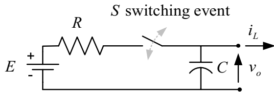
Figure 1 Power conditioning device.
