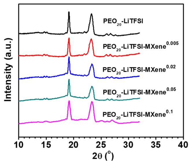
Fig. S1. WAXD patterns for PEO 20 -LiTFSI and CPEs with different MXene content.
