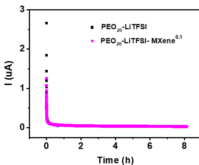
Fig. S2. DC polarization curves for PEO 20 -LiTFSI and PEO 20 -LiTFSI-MXene 0.1 at 60 °C.
