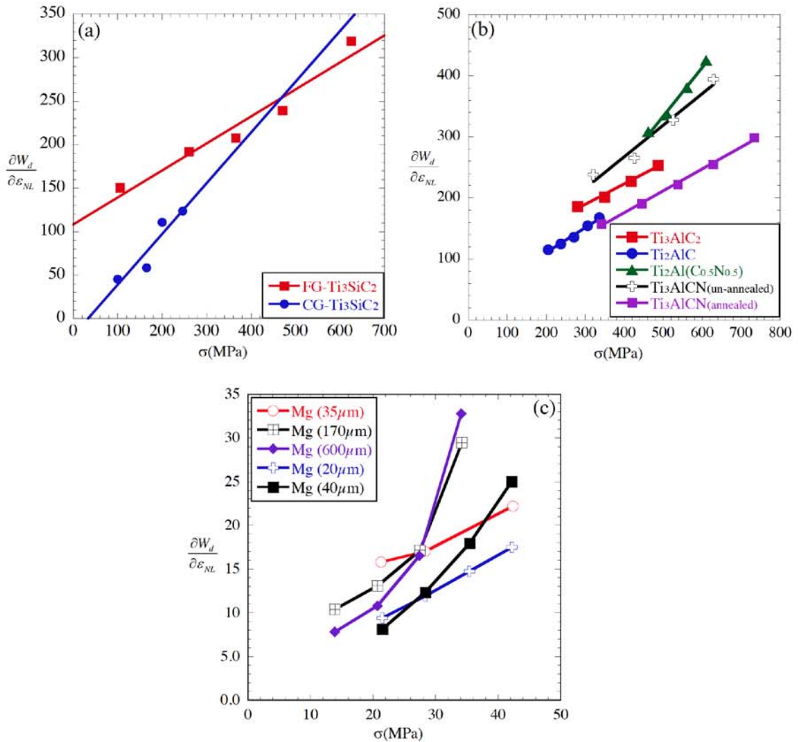
Fig. 3.6. \frac{\partial W_d}{\partial \varepsilon_{NL}} vs. \sigma plots for (a) FG- and CG-Ti 3 SiC 2 [77], (b) Ti 3 AlC 2 , Ti 2 AlC and Ti 3 AlCN [45], (c) pure Mg with different grain size [56]. The numbers in parantheses represent Mg grain size.
