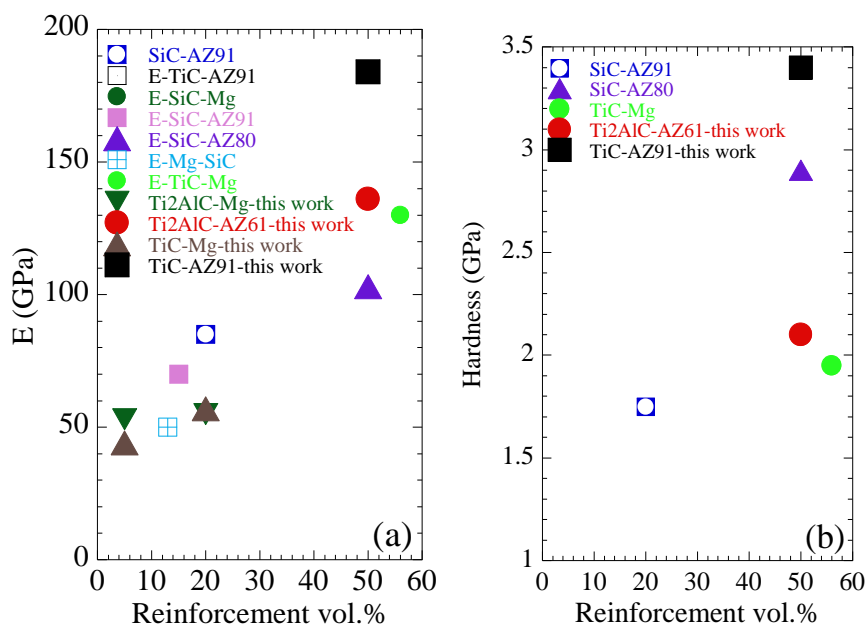
Fig. 5.16. (a) Highest elastic moduli of Mg composites reported in the literature are compared with E^* of FG50- Ti_2AlC -AZ61 and FG50- TiC -AZ91 and 5 and 20 vol.% reinforcement pure Mg composites; (b) the same comparison was done for the Vickers hardness values.
