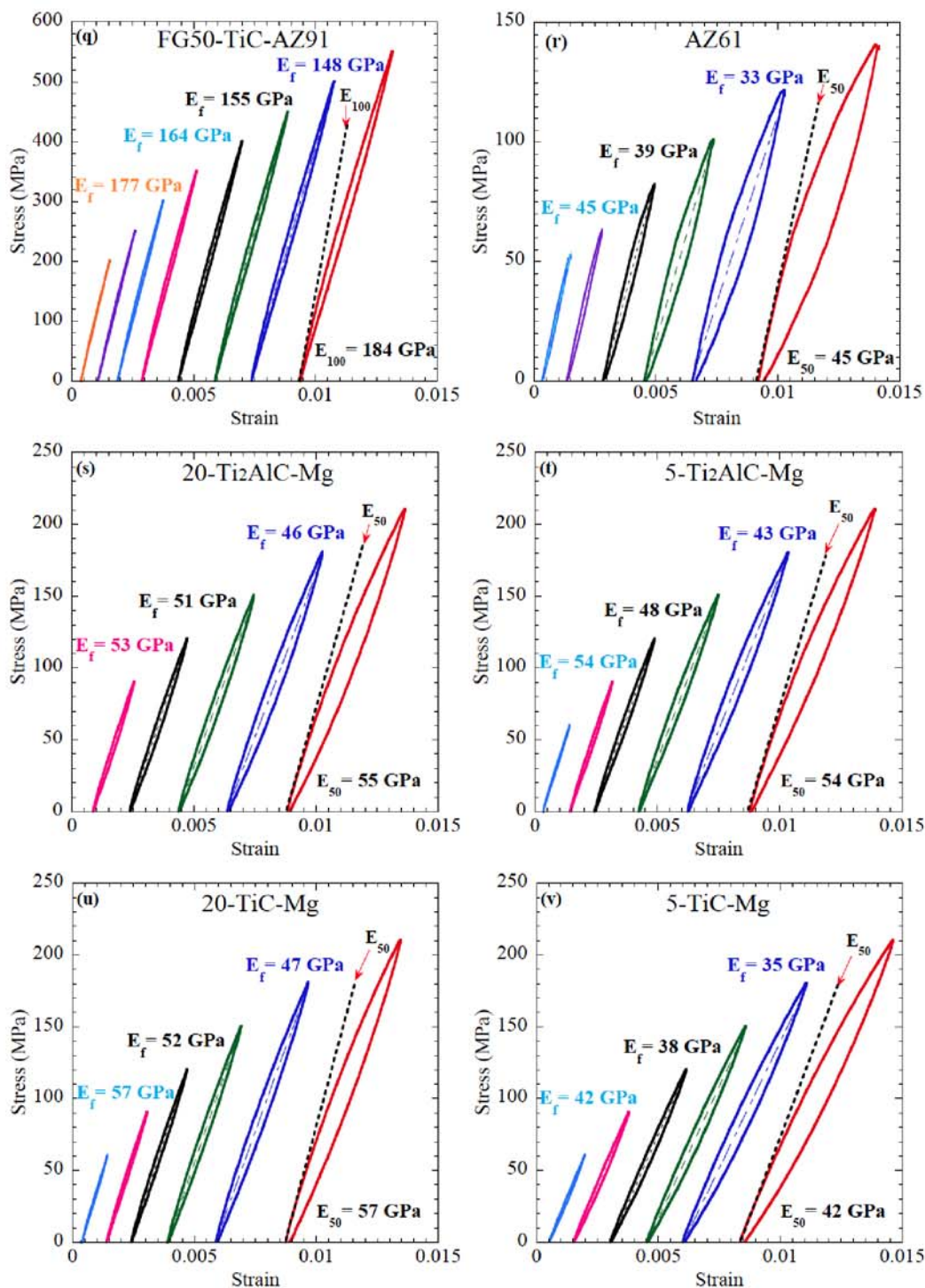
Fig. 6.2. (a) to (v) stress-strain cycles at various stresses for all the composites fabricated in this study. The curves are shifted horizontally for clarity. E_f (dashed lines inside the loops) are computed by least squares fits of the entire data set of each loop. E_{100} and E_{50} are the slopes of the stress-strain curves up to 100 MPa and 50 MPa, respectively.
