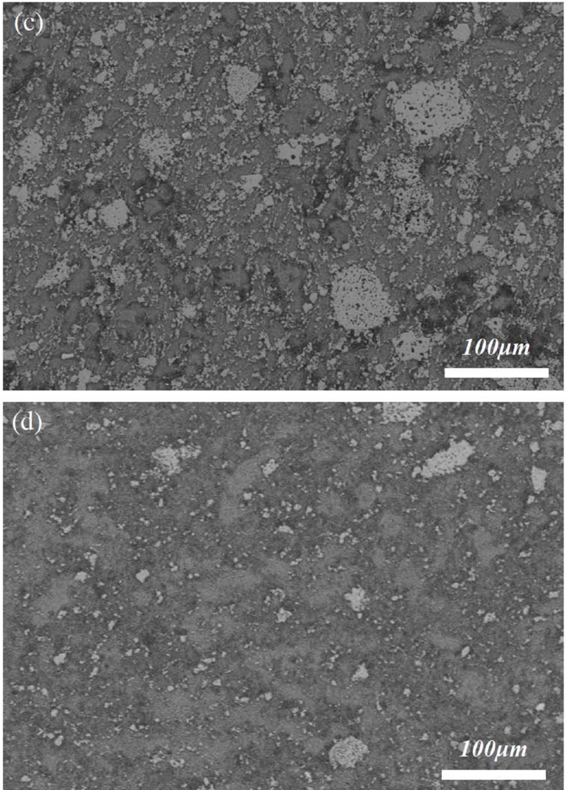
Fig. 5.1. Backscatter SEM micrographs of polished surfaces of: (a) 20-Ti 2 AlC-Mg, (b) 5-Ti 2 AlC-Mg, (c) 20-TiC-Mg, (d) 5-TiC-Mg composites.
