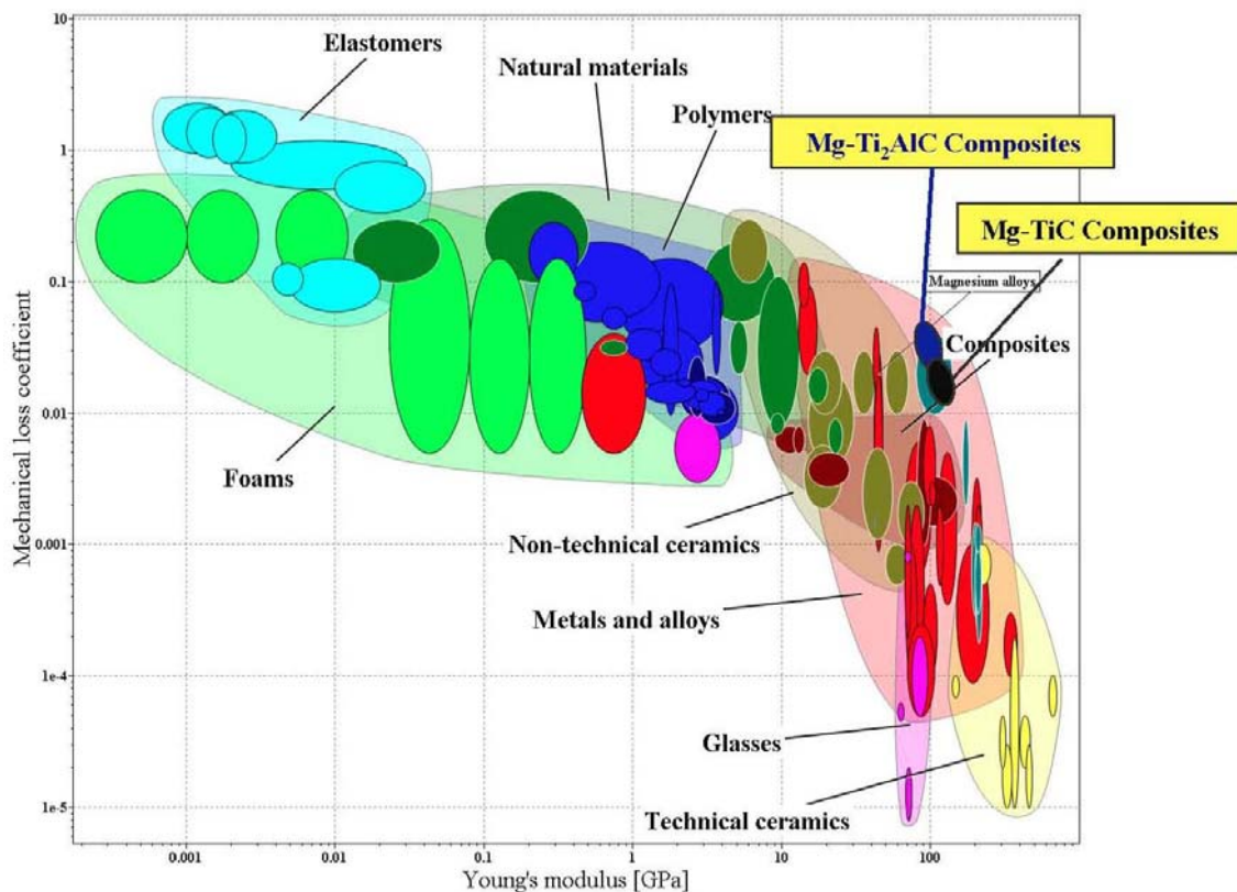
Fig. 6.10. Ashby map showing the log-log relationship between damping and Young's moduli of solids. The Ti_2AlC -Mg and TiC-Mg families of composites are shown in this map. Mechanical loss coefficient is calculated as W_d/2\pi U_{tot} [113].
