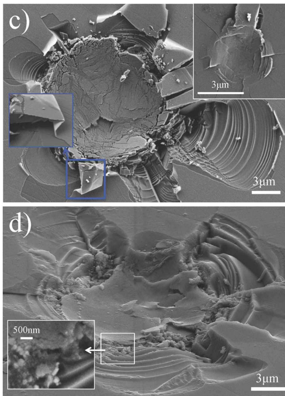
Fig. A1.S 1. SEM images of indentation marks on LiTaO 3 made with a 21 μm tip loaded to 550 mN, a) 5, b) 20, c) 40 and d) 100 times. The features with very sharp radii of curvature in (b) and (c) are kink boundaries. Top right inset in (c) shows the indentation mark made with a 5 μm tip loaded to 100mN for 40 times. Bottom left inset in (d) shows submicron grains that formed under the nanoindenter.
