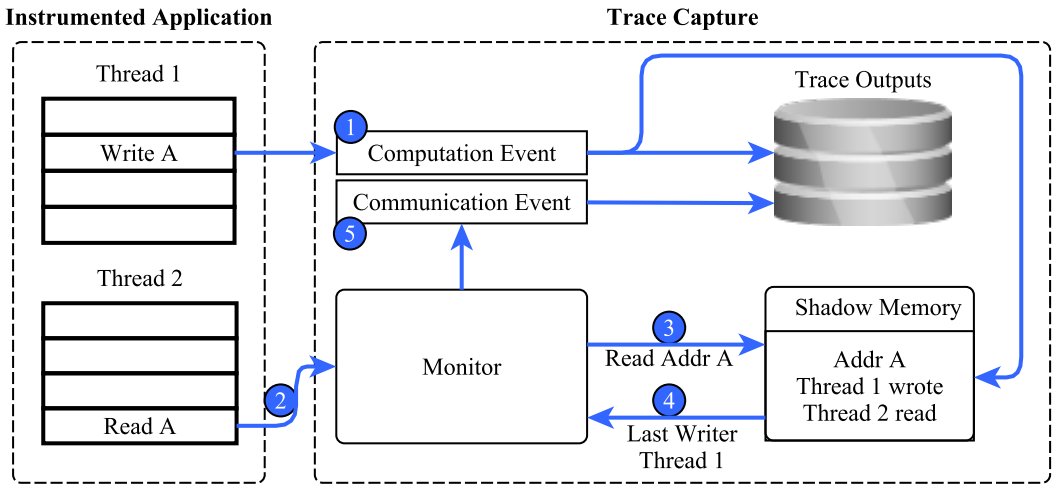
Fig. 4. Capturing Computation and Communication Events
