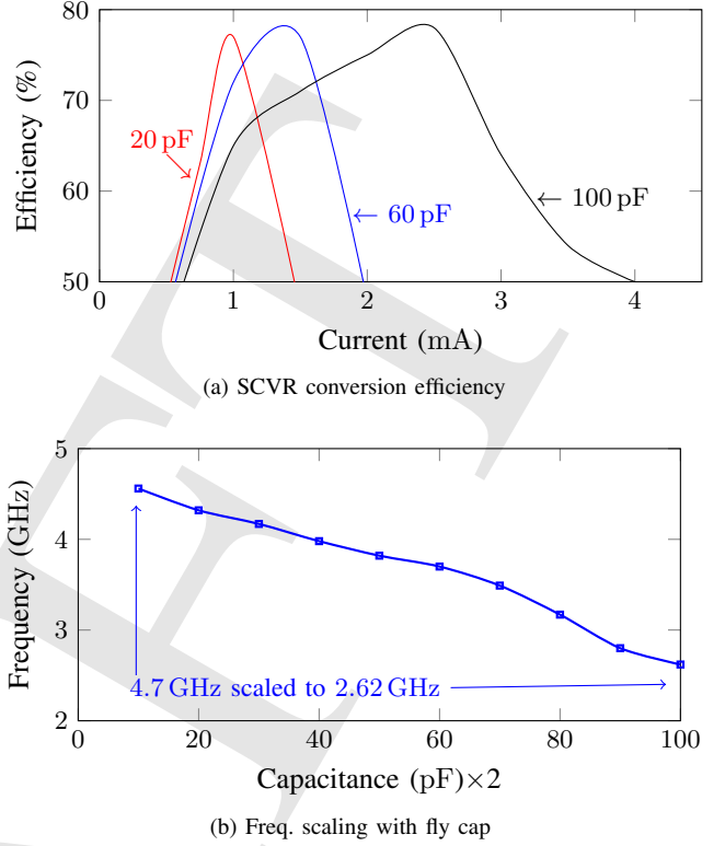
Fig. 10. Power conversion efficiency of SCVRs and frequency scaling of ReRoC with fly caps.
